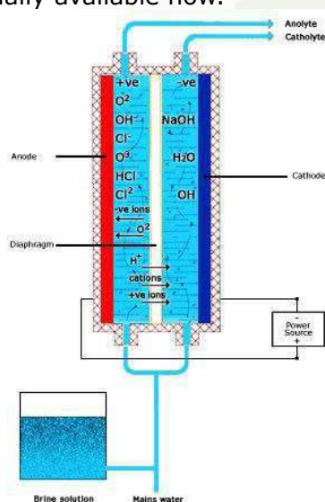
Design of Enviolyte cell
